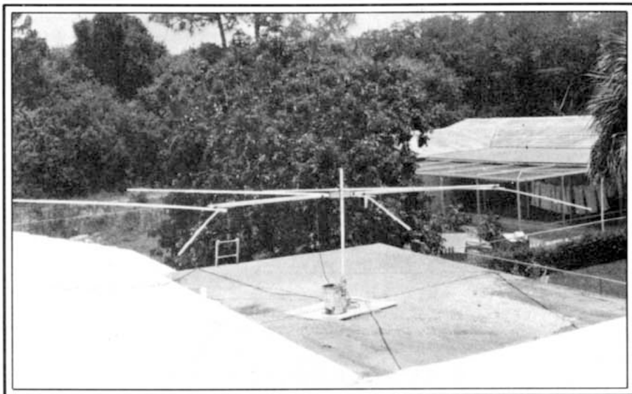
The second antenna features 3 elements on 15 meters at a height of 14 feet. Elements are swept forward at a 40° angle.
