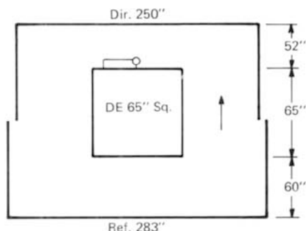
Fig. 1— A half-wave square loop with semi-square reflector and director.
